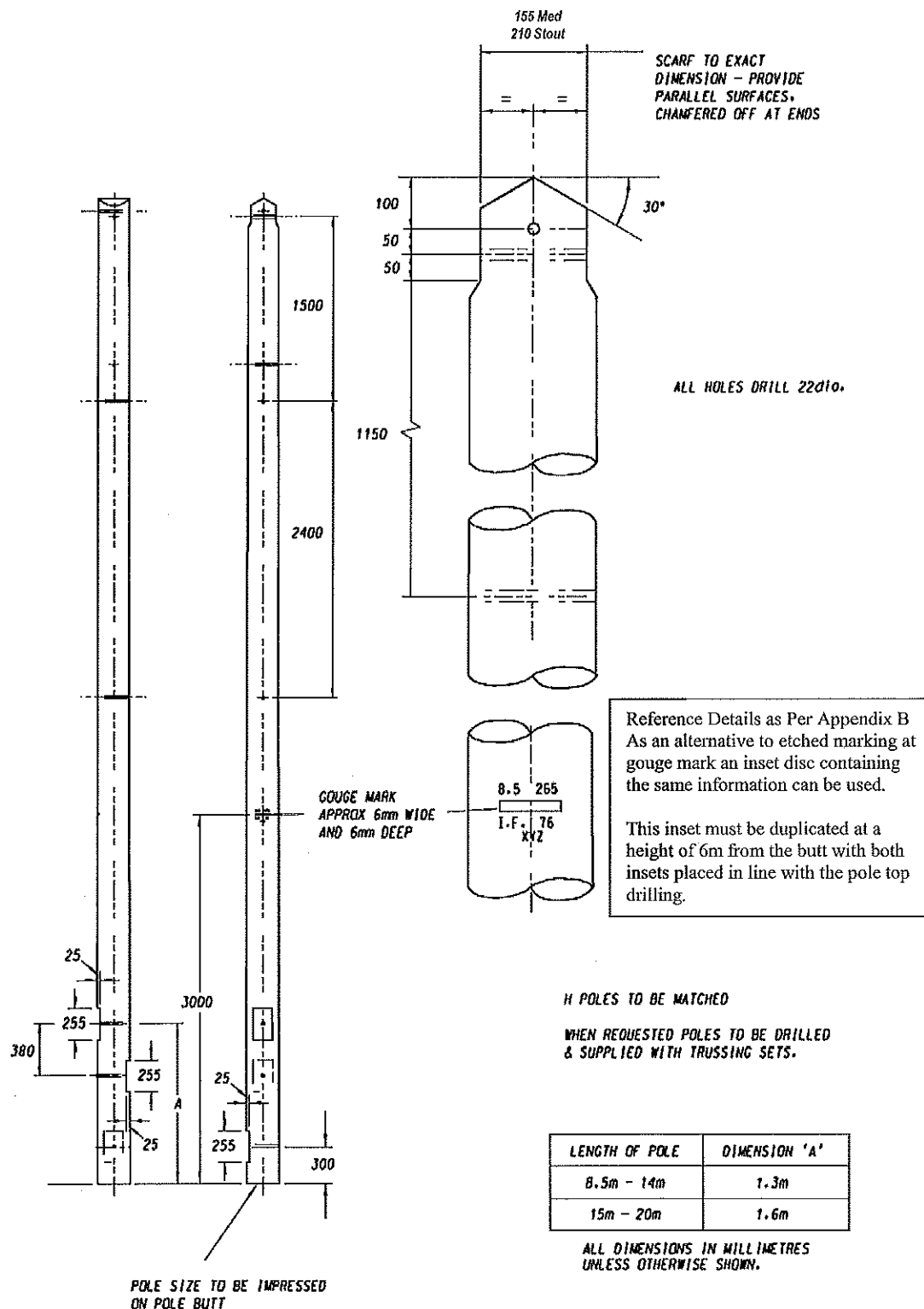
OH4T Fig 2 - H Pole Drilling, scarfing & Marking
